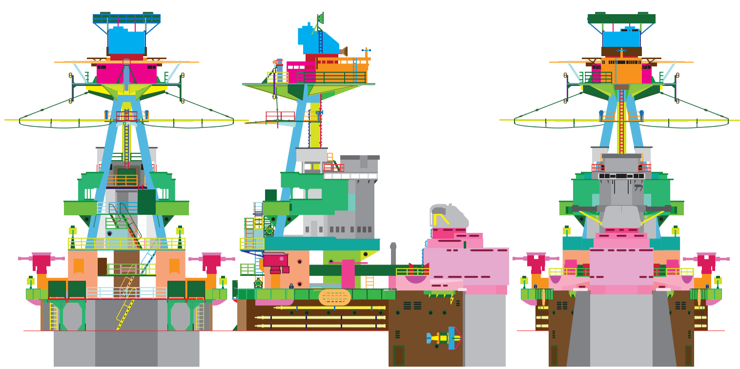
< Aft Searchlight Control Superstructure >
