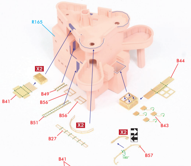
< Aft Searchlight Control Superstructure >
