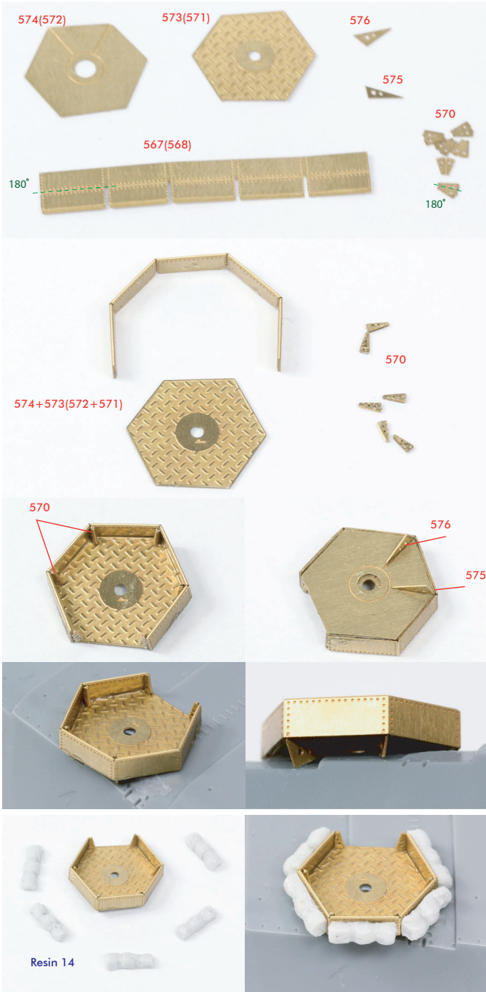
< A15(A16)の代替部品 2: A15(A16) Replacement >
