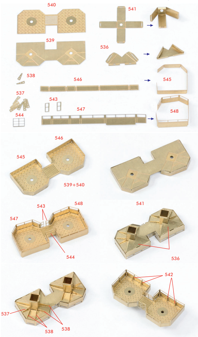
< A16(A15)の代替部品 1: A16(A15) Replacement >
