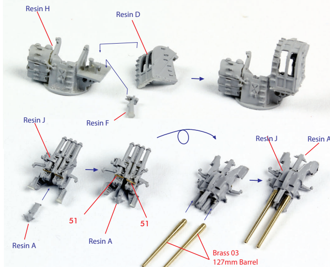
<12.7cm 連装高角砲 : 12.7cm High Angle Double Guns> < 37003F1/35003F2 IJN Yamato Detail Set only>
