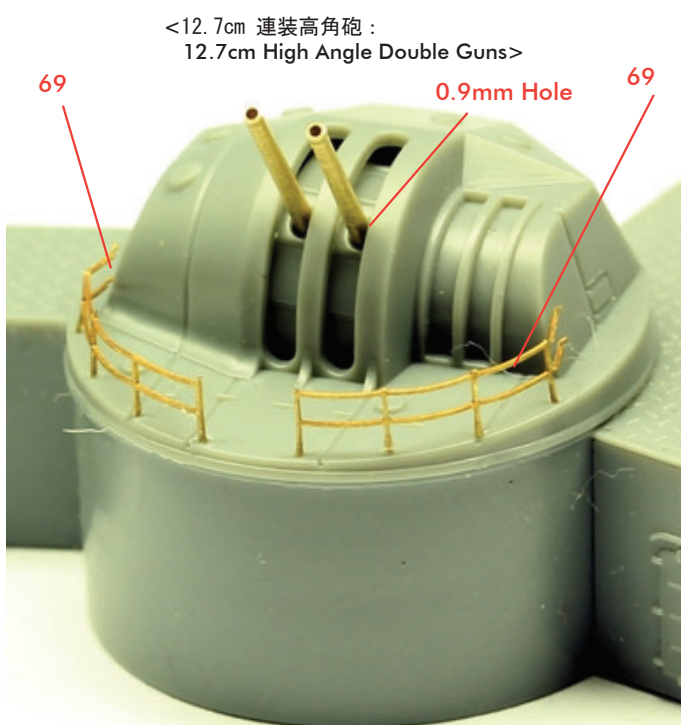
<12.7cm 連装高角砲 : 12.7cm High Angle Double Guns> < 37003F1/35003F2 IJN Yamato Detail Set only>
