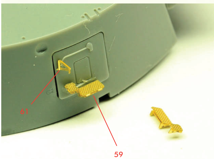
<弾薬箱: 25mm Ammunition Box>
