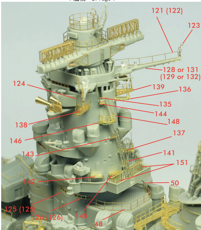
< 艦橋: Bridge >
