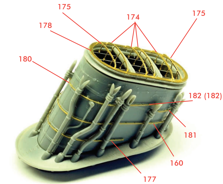
< 煙突: Funnel >
