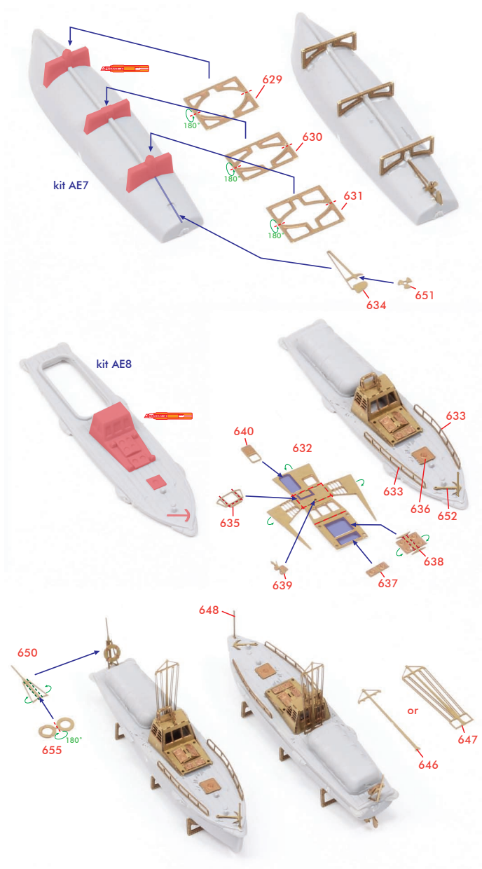
< 11m内火艇：11m Motor Boat >
