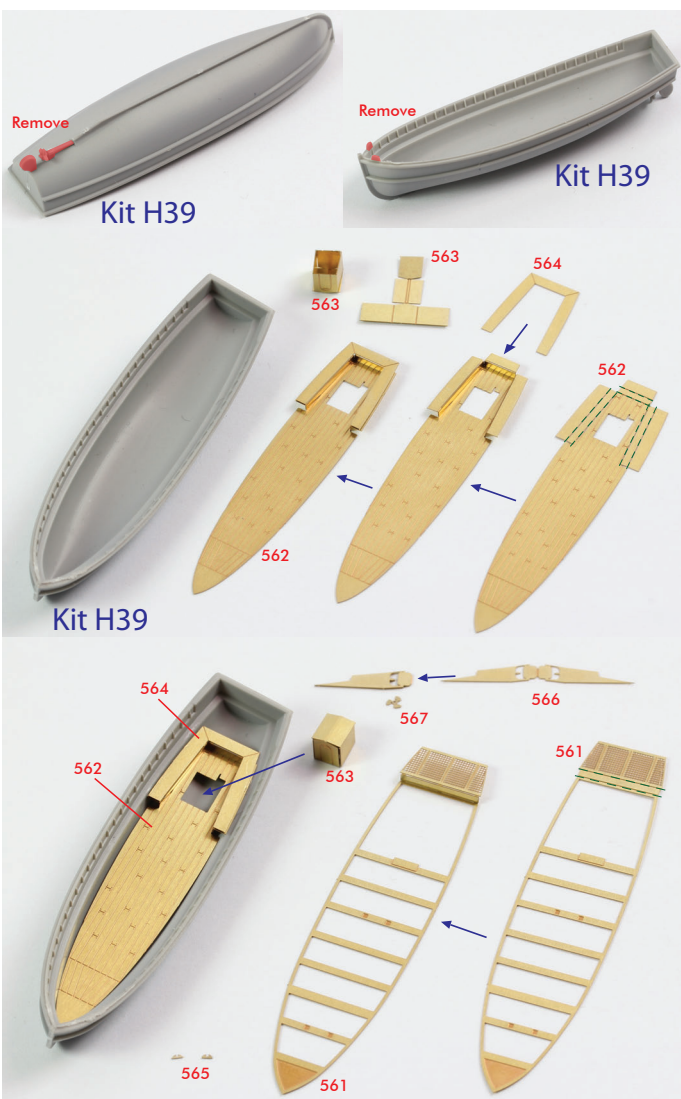
<45ft Motor Launch>
