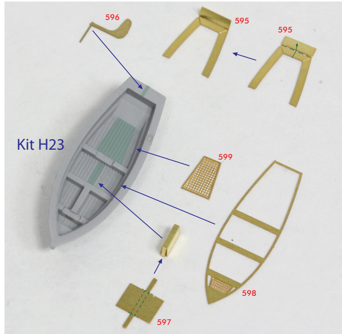
<16ft SAILING DINGHY>
