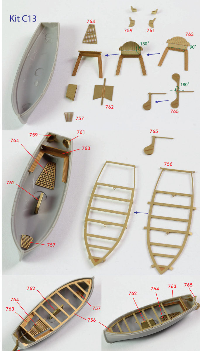
< 32ft. Cutter >
