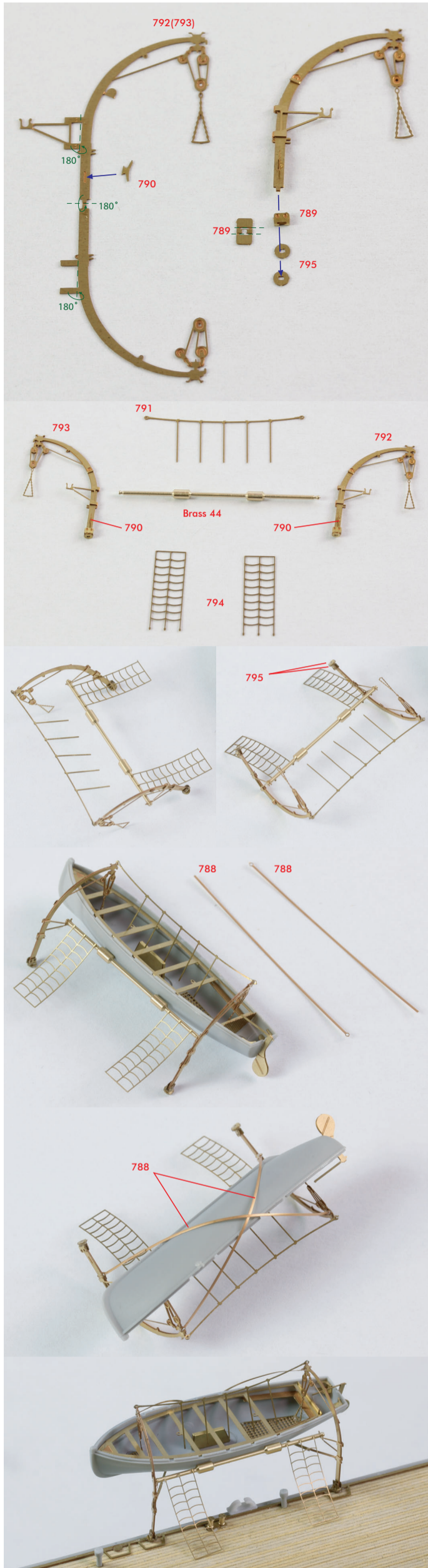
< Boat Davit >
