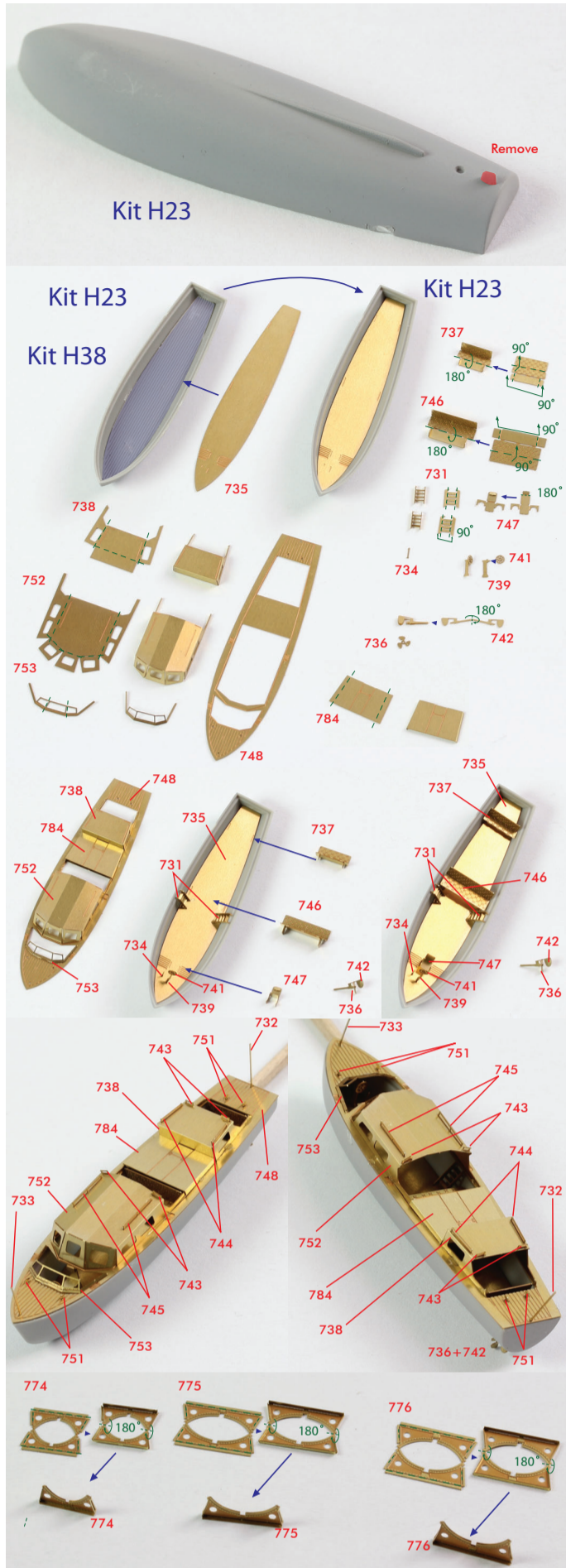
< 32ft. Cutter >
