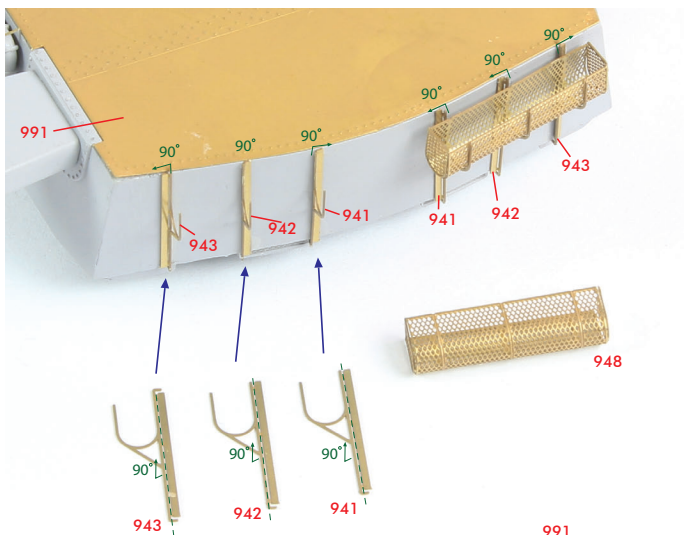
No.1 Turret
