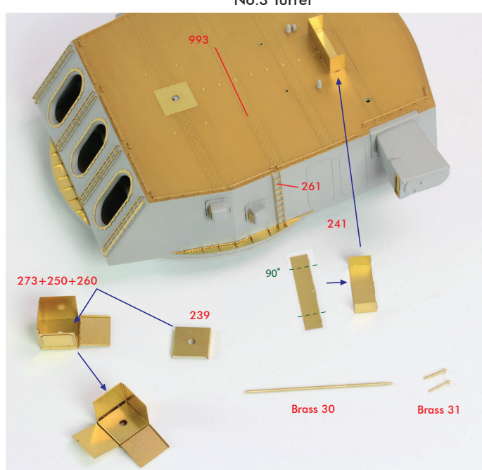
No.3 Turret
