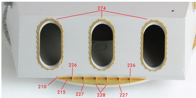
No.2 Turret
