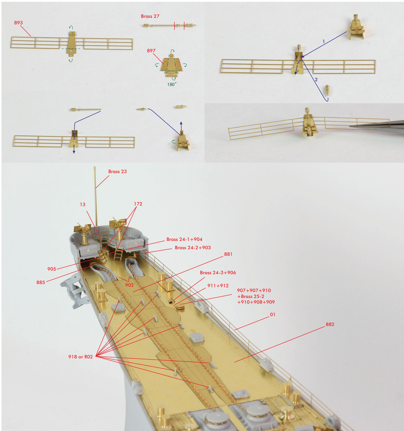
<Stern Lights>
