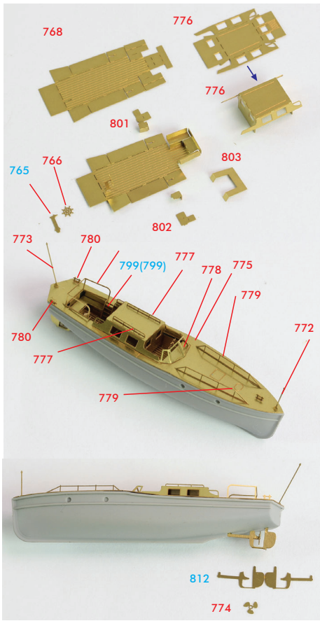
<Boat L30>
