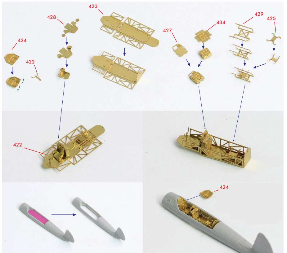
<Wing Folding>
