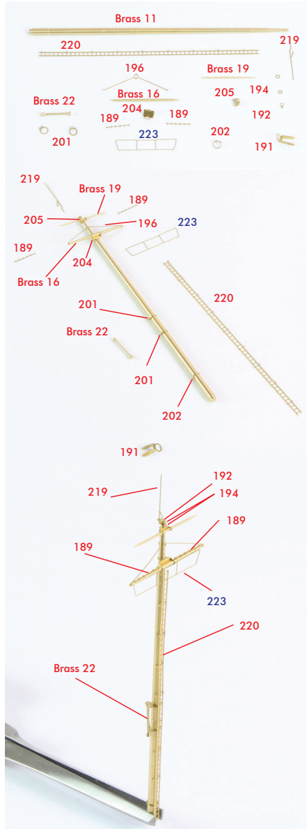
<Fore Mast>
