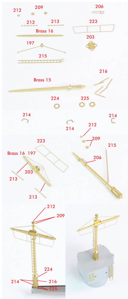
<Main Top Mast>
