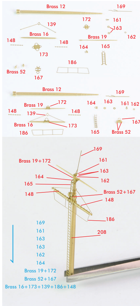
<Main Mast Base>
