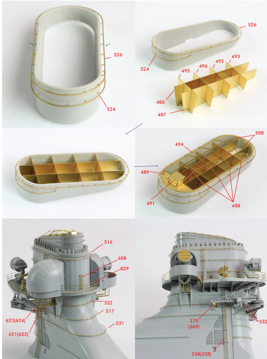
<Funnel>
