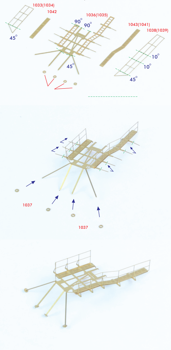
<Wire Stand on the Bow>
