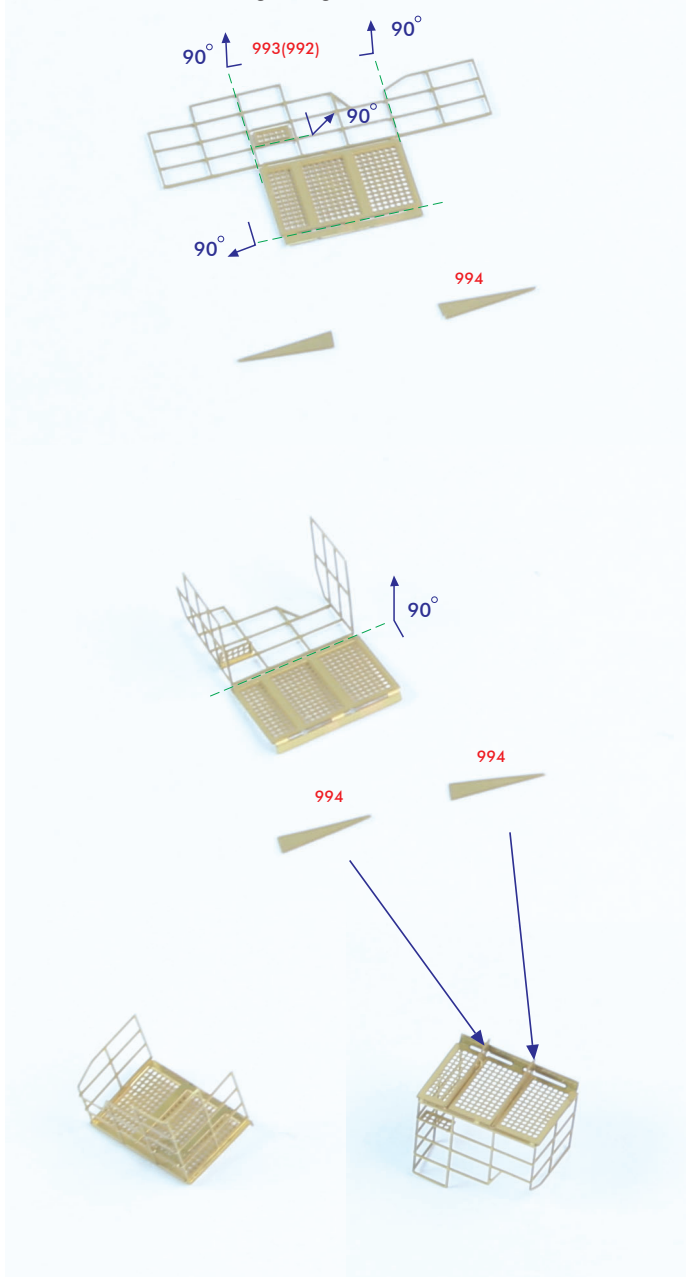
<Signal Light Guard Rails>
